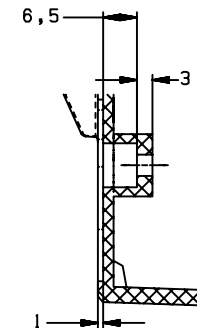
SECTION B - B
