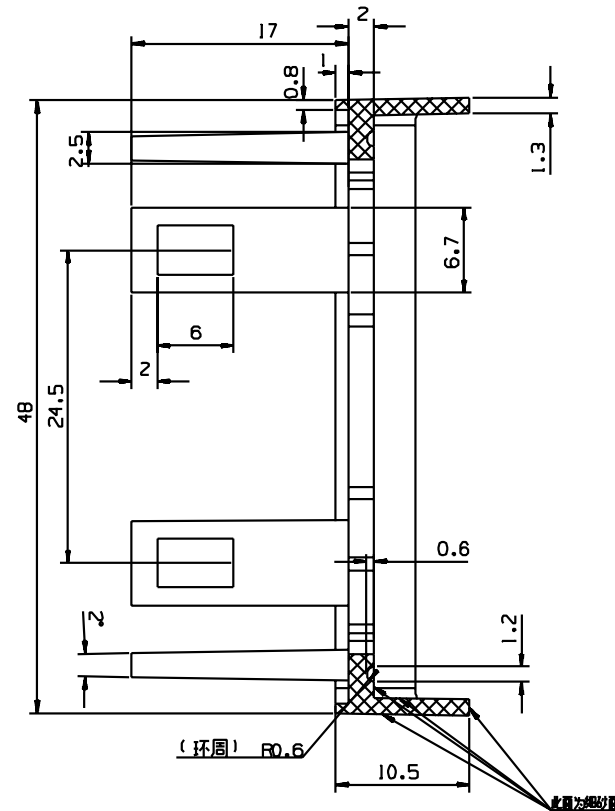
SECTION A-A SCALE 5:2
