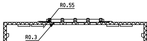
SECTION B - B
