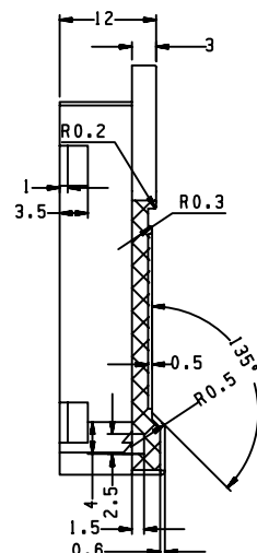
SECTION B-B
