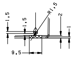
DETAIL E SCALE 1/1
