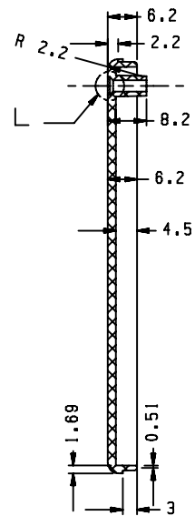
SECTION K - K
