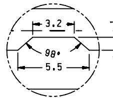
DETAIL J SCALE 5/1
