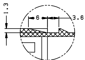
DETAIL E SCALE \frac{2}{1}
