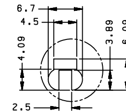
DETAIL C SCALE \frac{2}{1}
