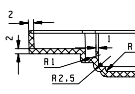
SECTION D - D
