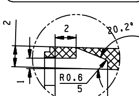
DETAIL E SCALE 4/1
