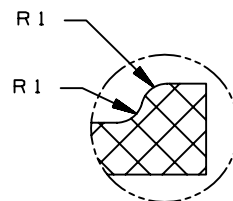
DETAIL C SCALE 5/1
