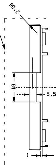
DETAIL D SCALE \frac{1}{4} "
