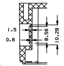
SECTION K - K
