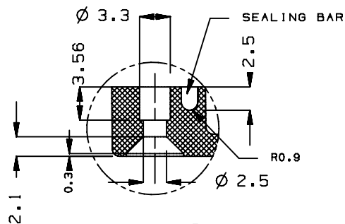
DETAIL C SCALE 1/10
